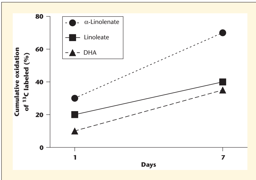
Figure 3. Slower beta-oxidation of ^{13}\text{C} -docosahexaenoic acid (DHA) compared to ^{13}\text{C} -linoleate and ^{13}\text{C} -alpha-linolenate over 1 and 7 d. Adapted from McCloy et al. (2004) and Plourde et al. (2011).
