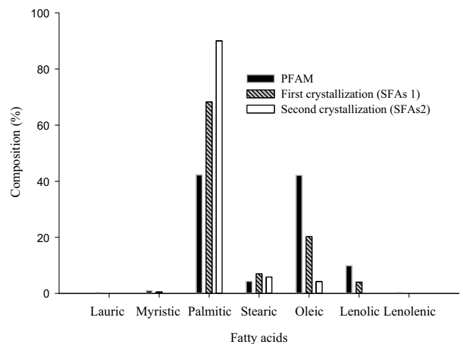
Fig. 4. Fatty acids profile of PFAM and SFAs before and after methanol crystallisation.
