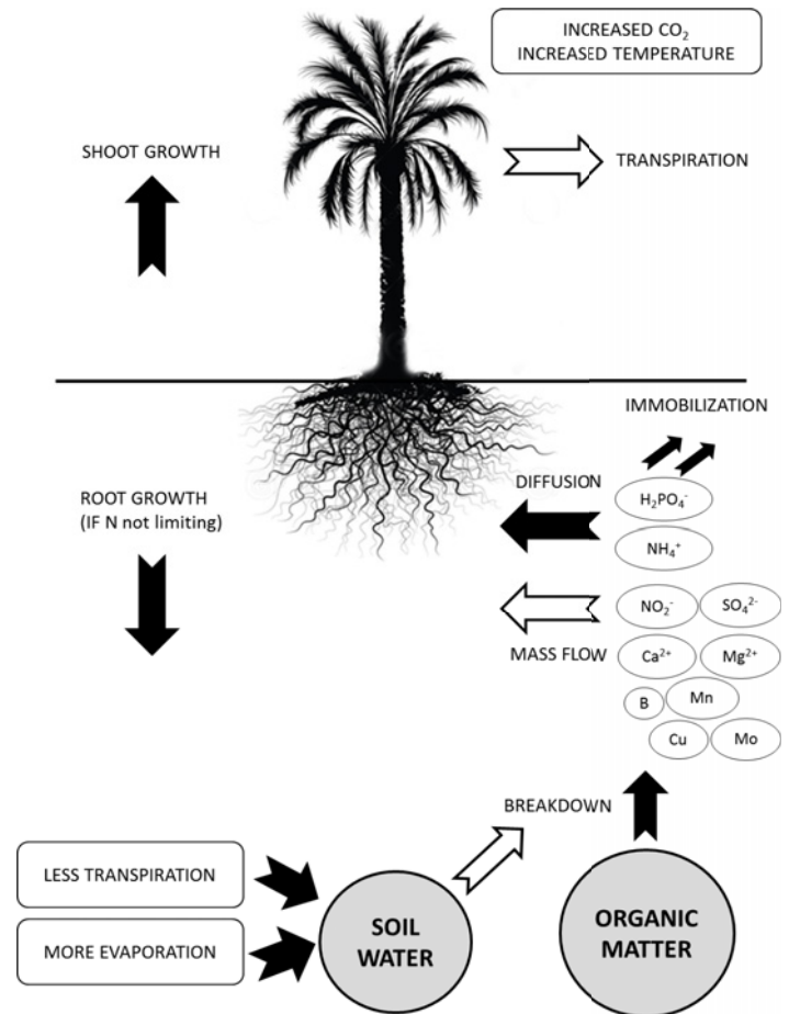
Fig. 2. Predicted effects of climate change on nutrient availability and plant growth. Variables affected by climate change are shown in boxes, and soil pools in circles. Decreases or increases in rainfall with climate change (dependent on geographic location) will interact with the effects of transpiration and evaporation on soil water pools. Mycorrhizal infection may increase with warmer temperatures, and lower effects of N and P limitation in nutrient-poor soils (adapted from Pilbeam, 2015).
